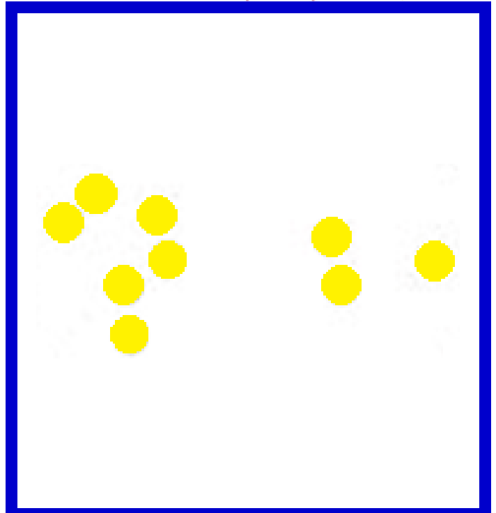
Leo
