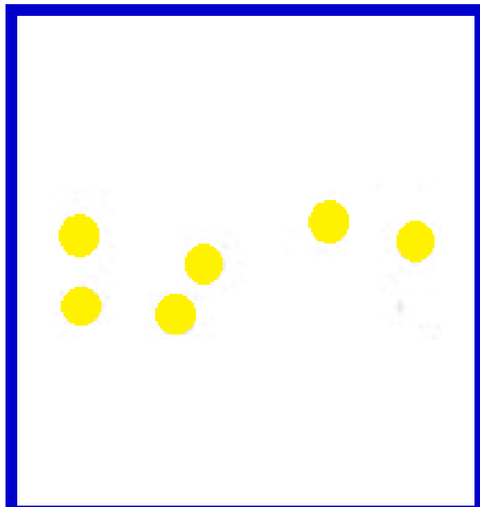
Osa Mayor
